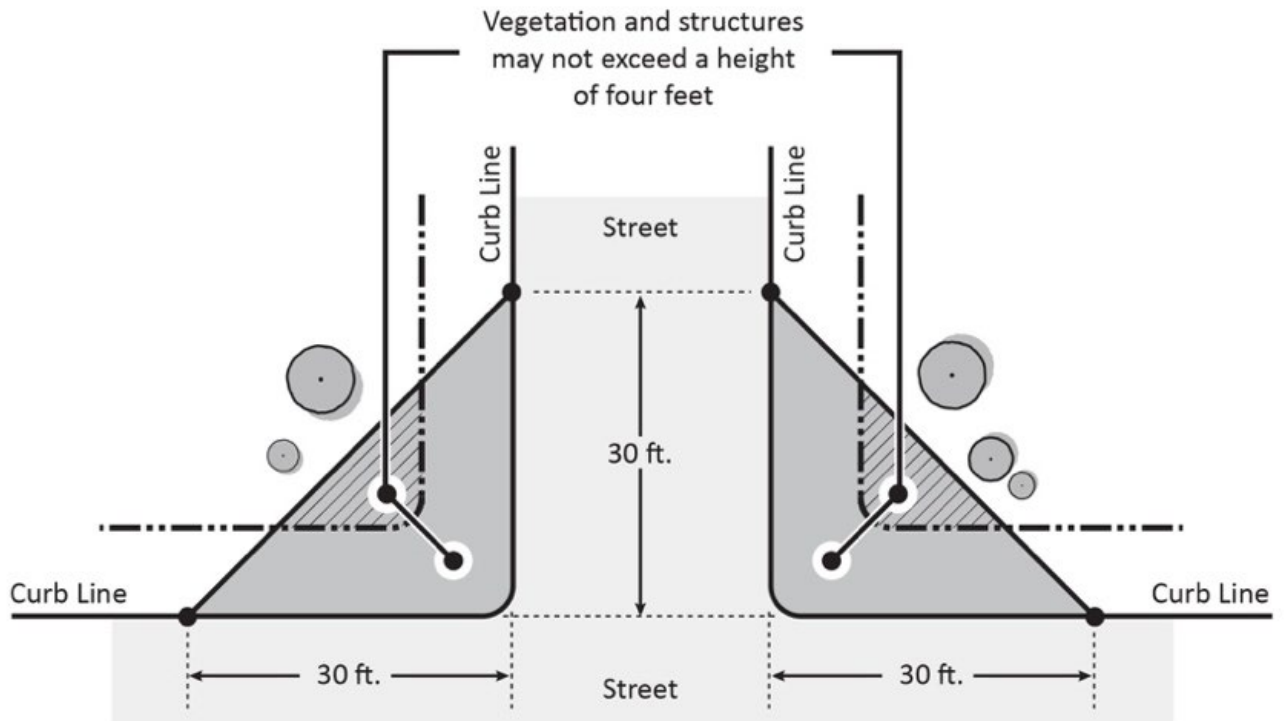
Figure 17.13.170-1 Visibility at Intersections.
