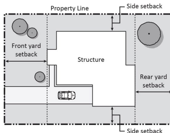
Figure 17.39.010-2 Required Yard.
