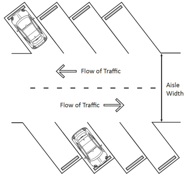
Figure 17.16.070-2: Aisle Dimensions
