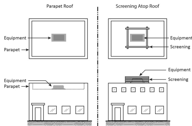
Figure 17.17.040-1 Rooftop Equipment Screening.
